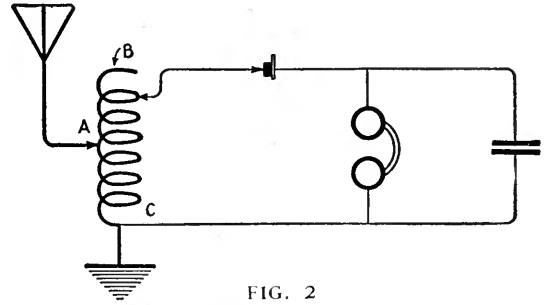
FIG. 2 A typical single-circuit receiver
