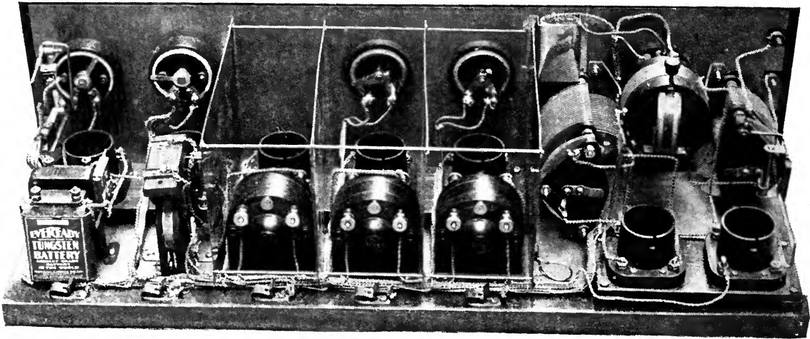
REAR VIEW, SHOWING METAL SHIELDING ENCLOSING THE INTERMEDIATE-FREQUENCY STAGES The layout may seem a bit complex, but none of the four parts which it comprises—wave-changer, I. F. amplifier, detector, A. F. amplifier—is particularly difficult to build. The circuit diagram, Fig. 1, shows clearly this division into parts
