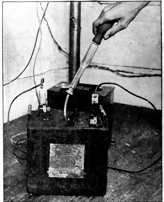
FIG. 5 Determining the state of charge of a battery with a hydrometer
