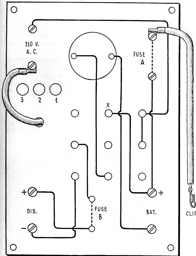
FIG. 3 Rear view of the panel
