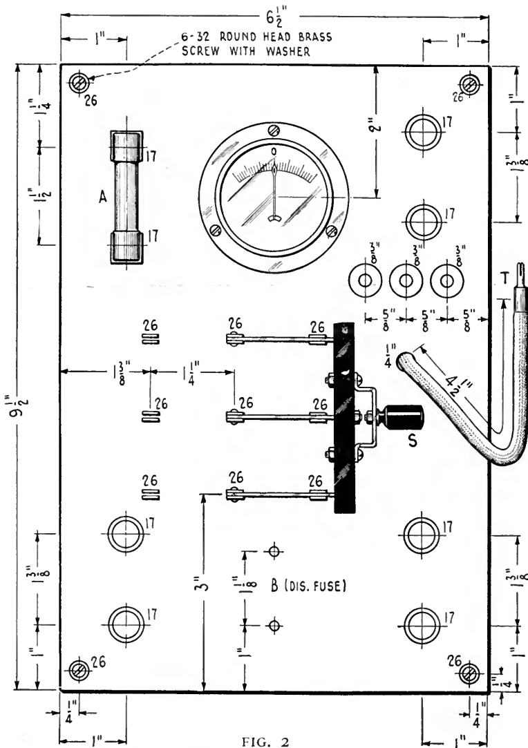
FIG. 2 A working drawing for the charger panel
