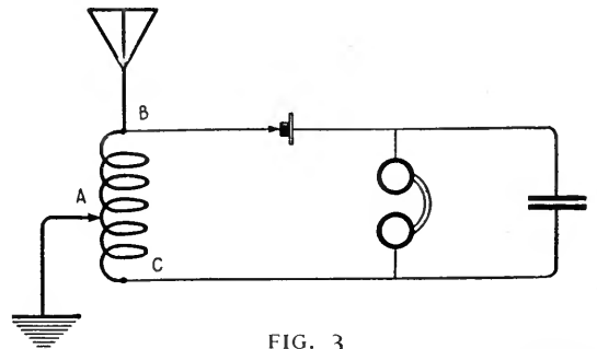
FIG. 3 An improvement over the arrangement shown in Fig. 2
